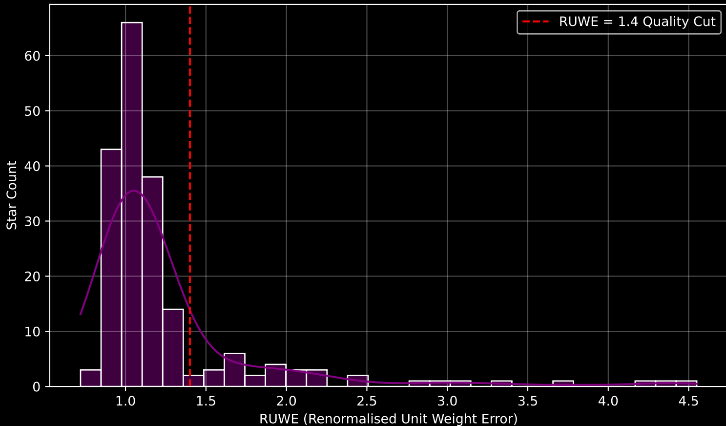
GAPOGEE DR17 Field [230+77_MGA] RUWE Distribution (n= 197)
