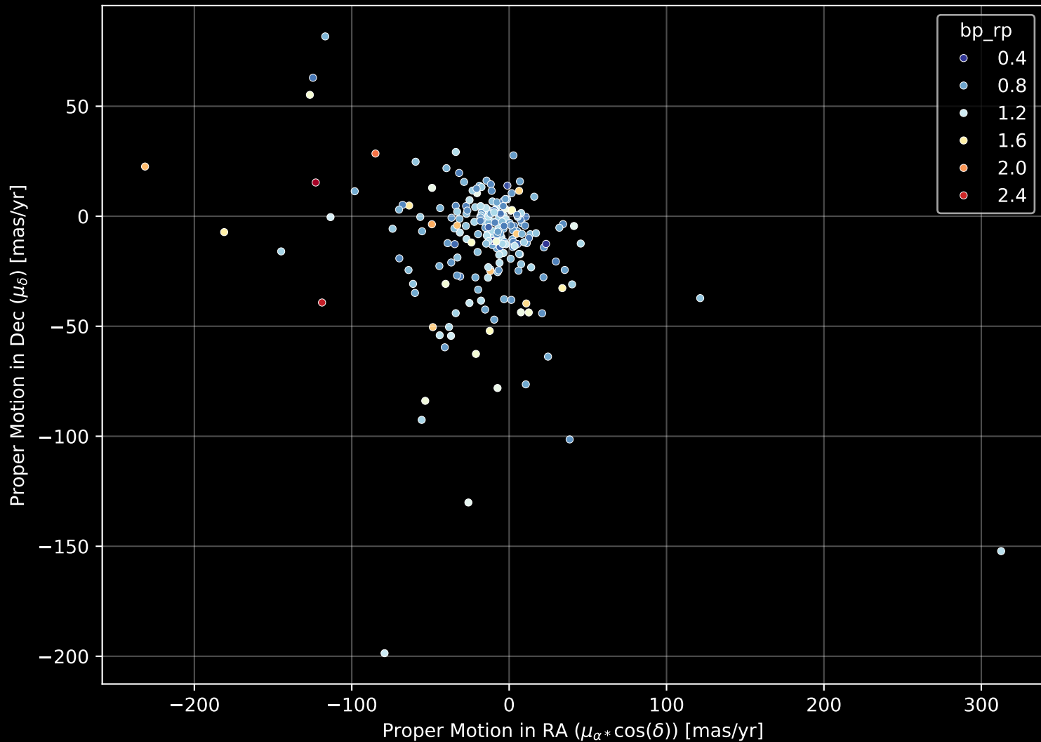
APOGEE DR17 Field: [230+77_MGA] Proper Motion Diagram (n= 212)
