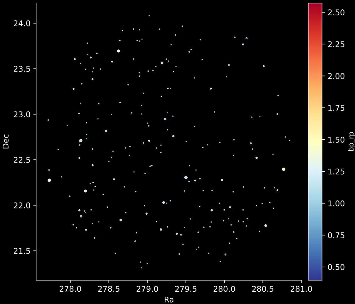
APOGEE DR17 Field: [230+77_MGA] Stars: 212
