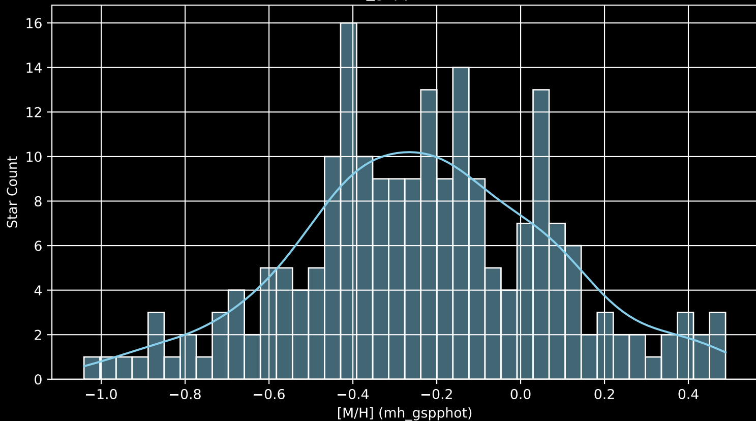
APOGEE DR17 Field: [230+77_MGA [M/H] (mh_gspphot) (n= 209)
