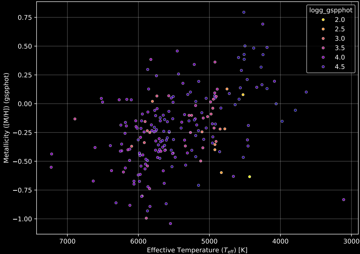
APOGEE DR17 Field: [230+77_MGA] Stellar Population Parameters (n= 212)
