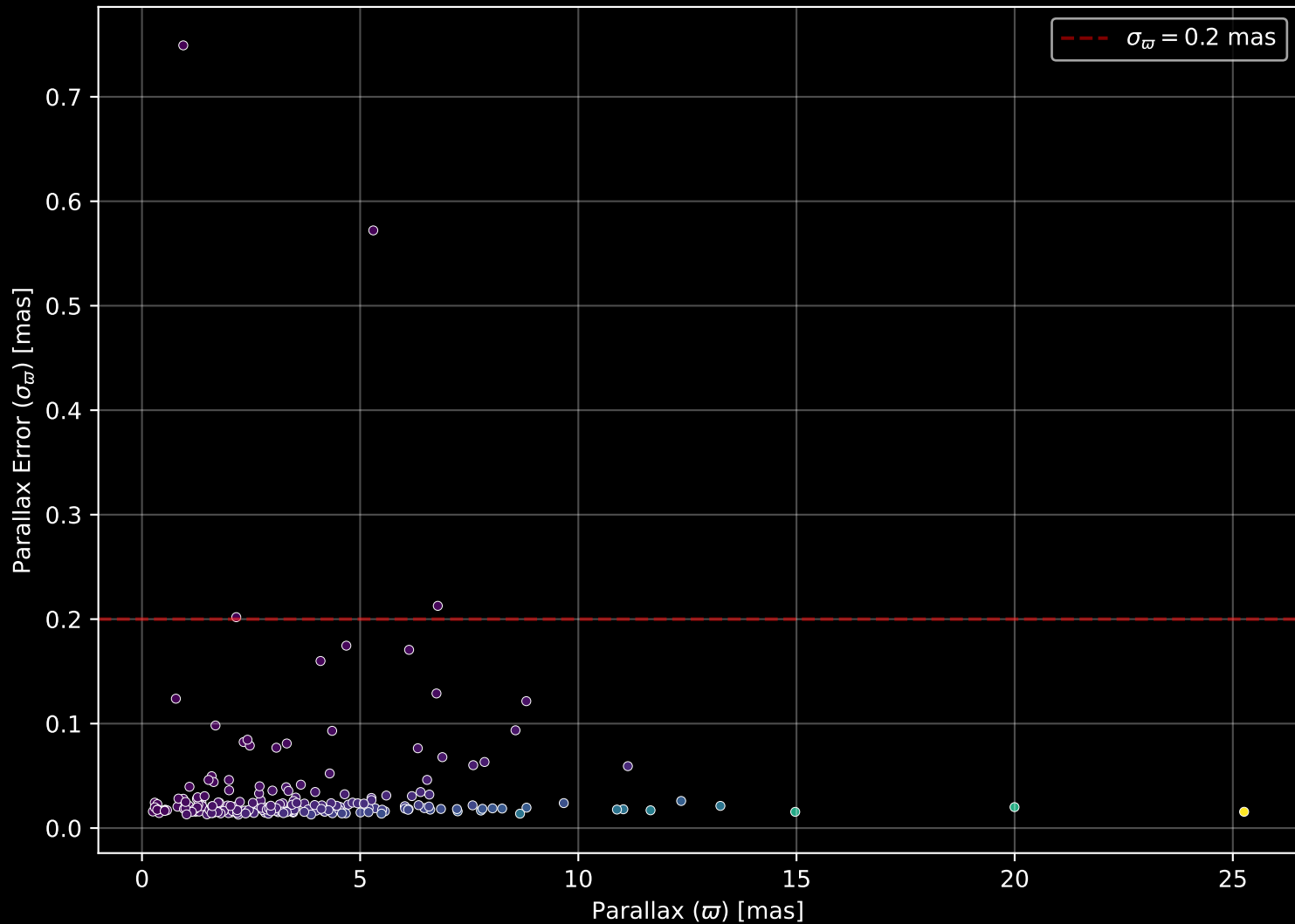
APOGEE DR17 Field: [230+77_MGA] Parallax Quality (n= 212)
