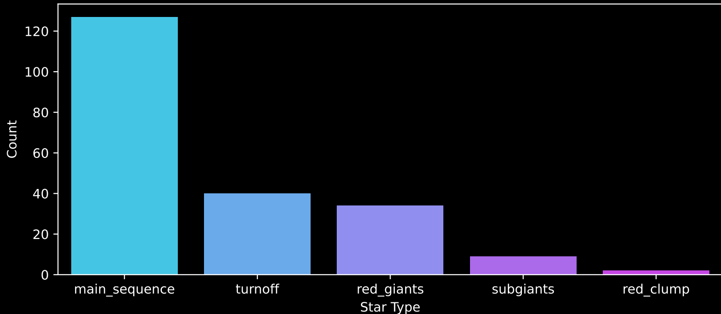
APOGEE DR17 Field: [230+77_MGA] Count plot of Star Type
